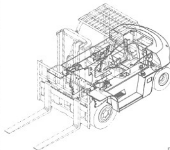
车架与平衡重 FRAME & COUNTER WEIGHT
