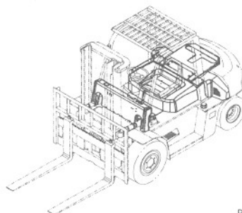
机罩、底板及座椅 HOOD, FLOOR BOARD & SEAT
